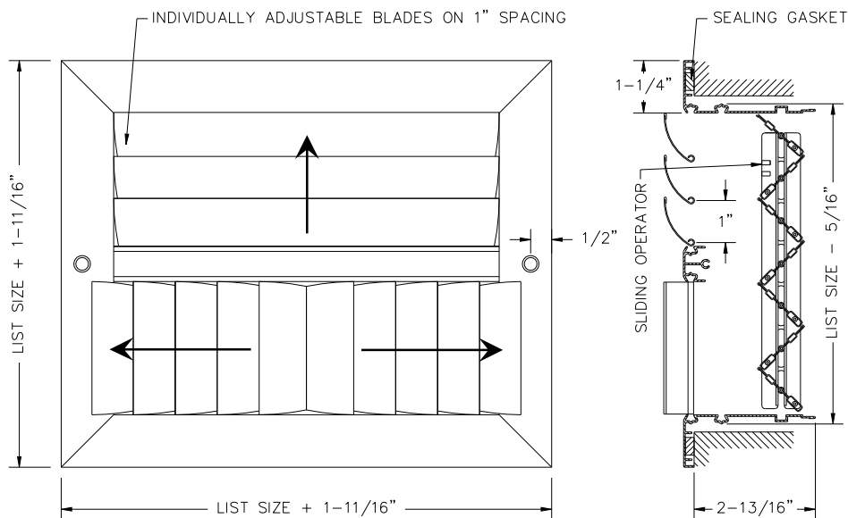
Standard blade option shown. See Curved Blade Options page.
